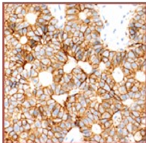
HER-2
