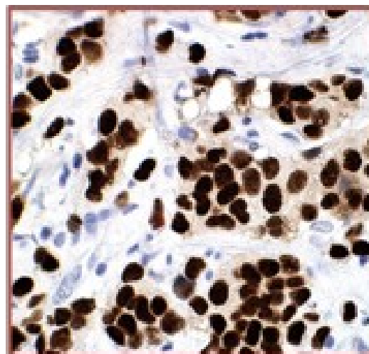
RE +
